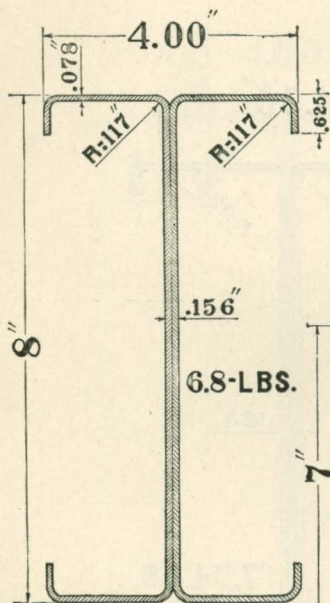
8"—6.8 lb. I Joist
