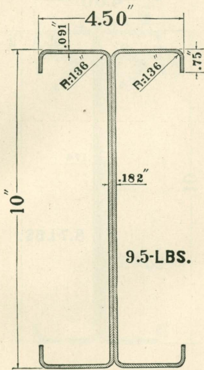
10" — 9.5 lb. I Joist
