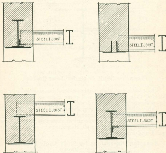
Details where steel joists are supported on Lintels in masonry walls.
