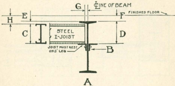
Locating Shelf Angle for Joist Bearing
