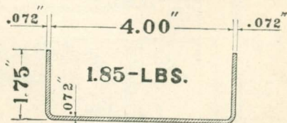
4"—1.85 lb. Partition Plate
