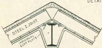
DETAIL AT-C Roof Construction Details of steel joist hip roof construction.
