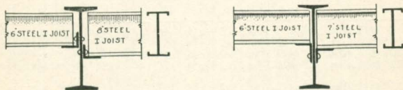
Steel Joists of different sizes set on shelf angles.
