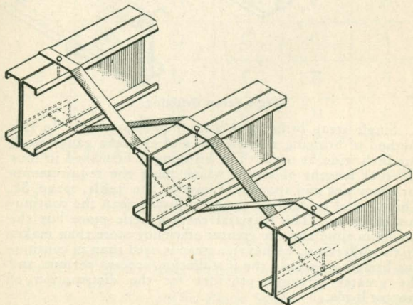
Continuous Bridging
