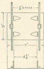
BEAM CLIP-B FOR 6'-9'-10'-11' & 12' STEEL JOIST
