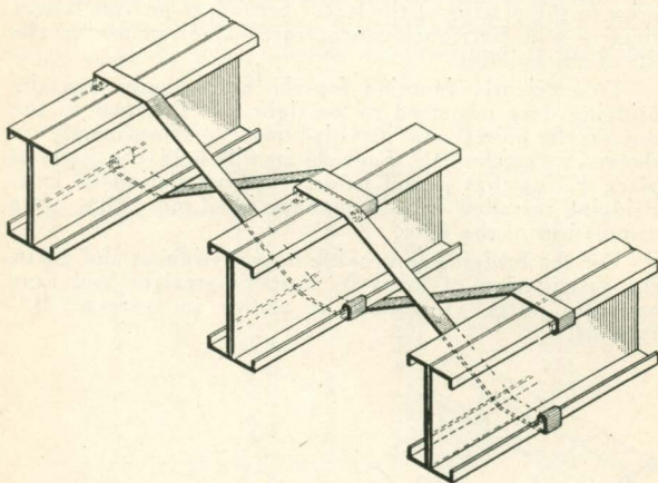
Single Strap Bridging
