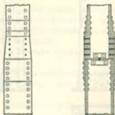
TYPICAL SPLICE
