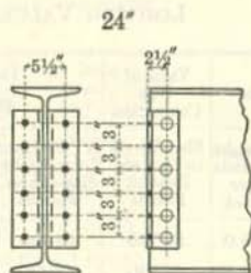
2 I 4 4" x 4" x 1/2" x 1'-5 1/2" Weight 39 lbs.
