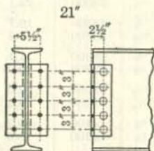
2 I 4 4" x 4" x 1/2" x 1'-2 1/2" Weight 33 lbs.
