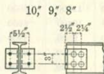
2 I 4 6" x 4" x 3/8" x 0'-5 1/2" Weight 13 lbs.
