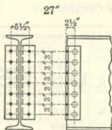
2 I 4 4" x 4" x 1/2" x 1'-3 1/2" Weight 46 lbs.
