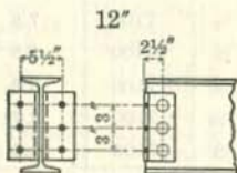
2 I 4 4" x 4" x 1/8" x 0'-8 1/2" Weight 17 lbs.
