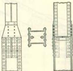
TYPICAL SPLICE
