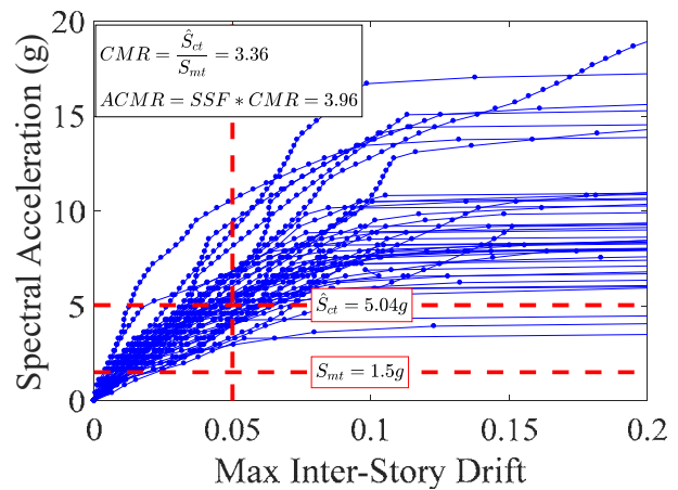
Figure 10-15. Fragility Curve (left) and Incremental Dynamic Analysis (IDA) (right) results of 3 story archetypes designed with: a) 63% coupling ratio (CR), b) 48% CR, c) 54% CR, d) 48.5% CR and; e) 32% CR
